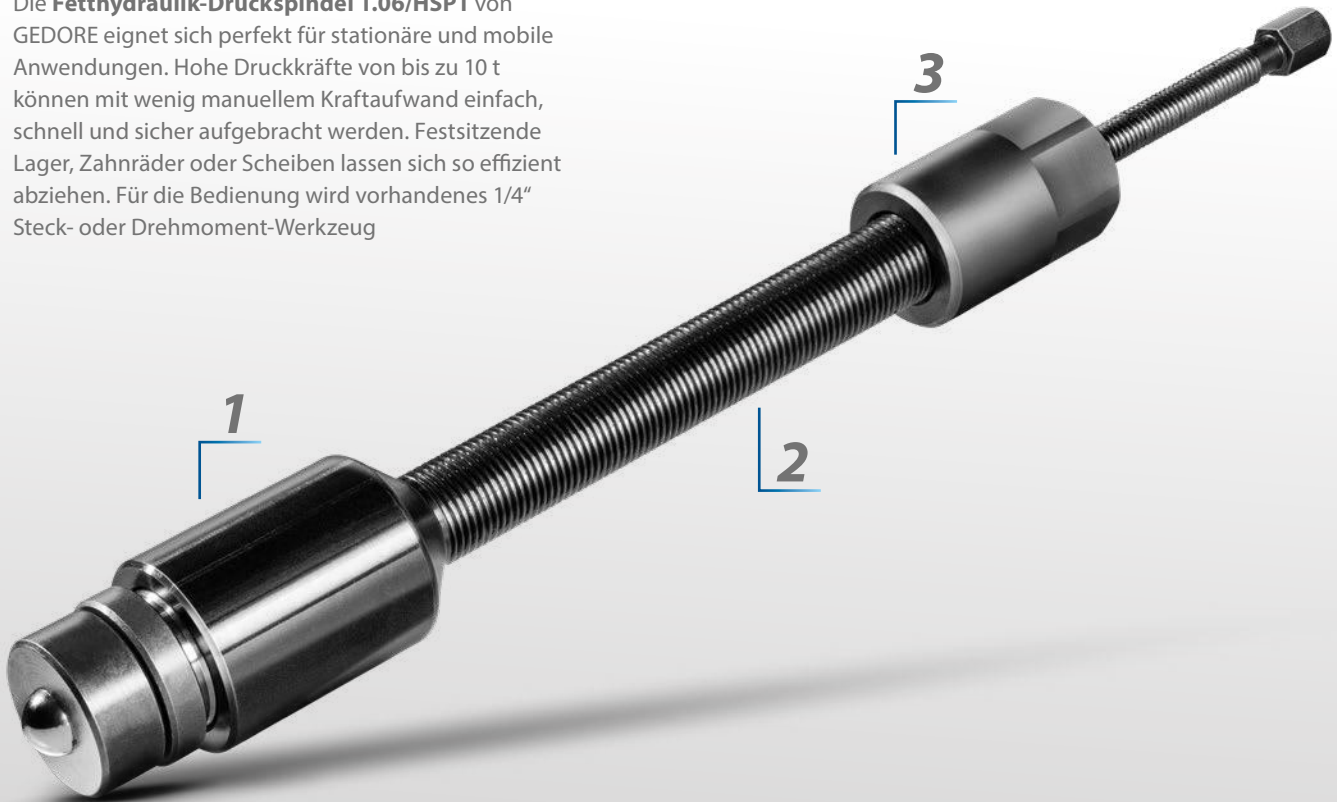
Fetthydraulik-Druckspindel 1.06/HSP1
